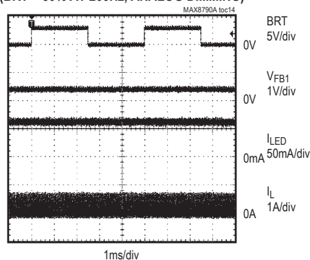
LED CURRENT WAVEFORMS (BRT = 50% AT 200Hz, ANALOG DIMMING)
