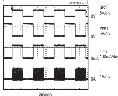
LED CURRENT WAVEFORMS (BRT = 50% AT 200Hz, DPWM DIMMING)
